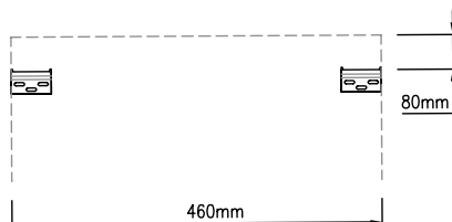
Fig. 1 - Square Under Basin Wall Bracket Set Out Detail
