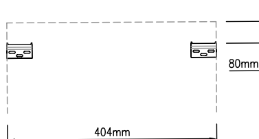
Fig. 1 - Square Under Basin Wall Bracket Set Out Detail
