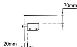
Fig. 3 - Set Out Detail for Furniture Brackets
